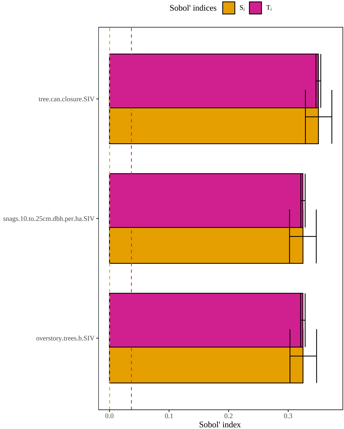
Figure 4. Results of a sensitivity analysis for the blackcappedchickadeeFoodCanH model based on an arithmetic mean structure. Dashed lines represent baseline numerical approximation error for S_i and T_i ( i.e. , dummy variables).
